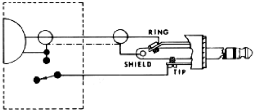
Figure 2-1. Microphone Connections
